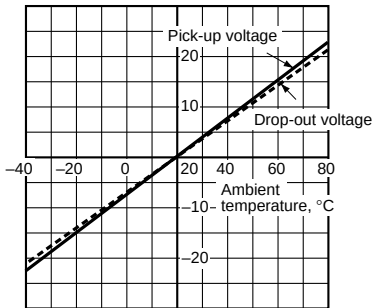
7. Ambient temperature characteristics
