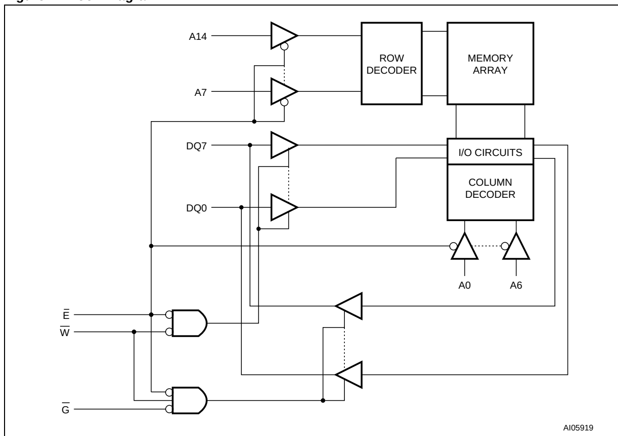
Figure 7. Block Diagram
